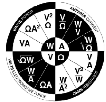
Ohms law wheel WVVOA
