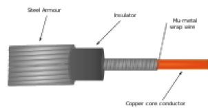
Mu-metal cable
