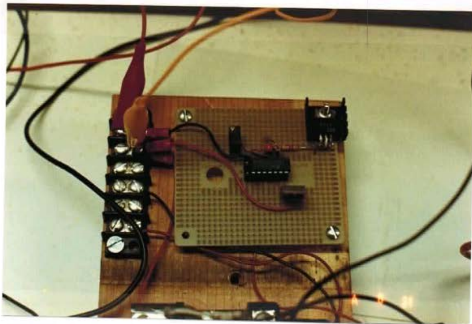
PICTURE 2 THE SOLID STATE TIMING DEVICE IN OPERATION
