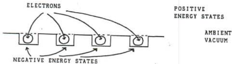
FIGURE 5. The Normally-Filled Dirac Sea
