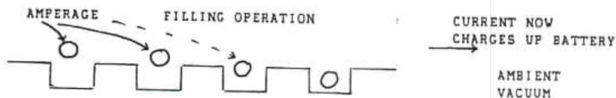
FIGURE 7. Filling The Dirac Sea Holes
