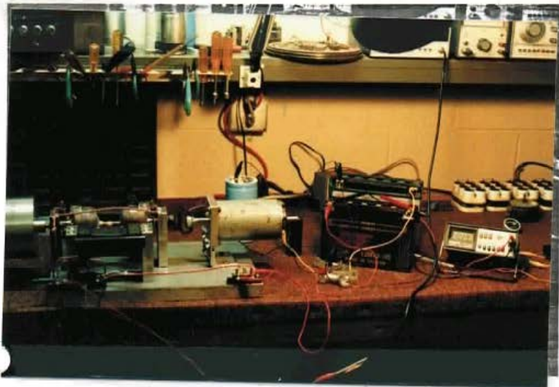
PICTURE C-1.1 KROMREY CONVERTER SECOND TEST SETUP
