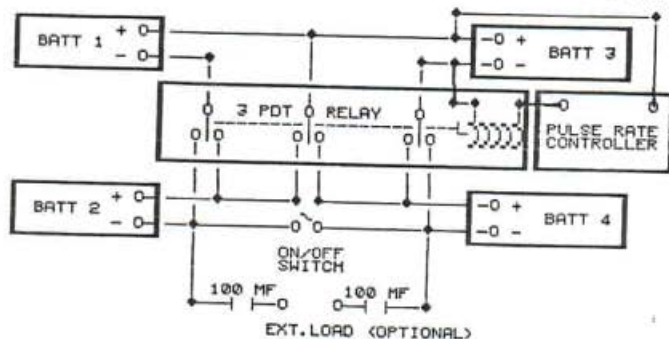
BEDINI, MUELLER, MOORE 23 AUGUST 1984 PICTURE 3 TESLA SWITCH - SIMPLIFIED DIAGRAM
