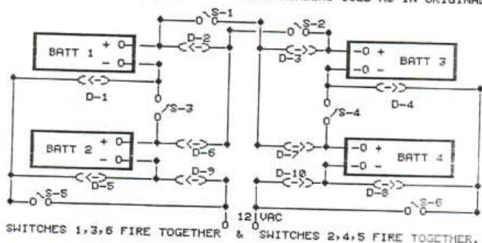
BEDINI, BRENTTE, MUELLER 23 AUGUST 1984 PICTURE 5 TESLA SWITCH SAME NUMBERS USED AS IN ORIGINAL
