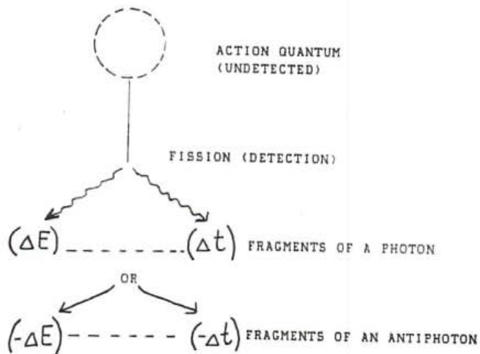
FIGURE 3. Two Possibilities of Action Quantum Fissioning
