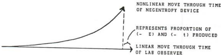
FIGURE 4. Production of Negentropy by Local Curvature of Spacetime Vacuum.
