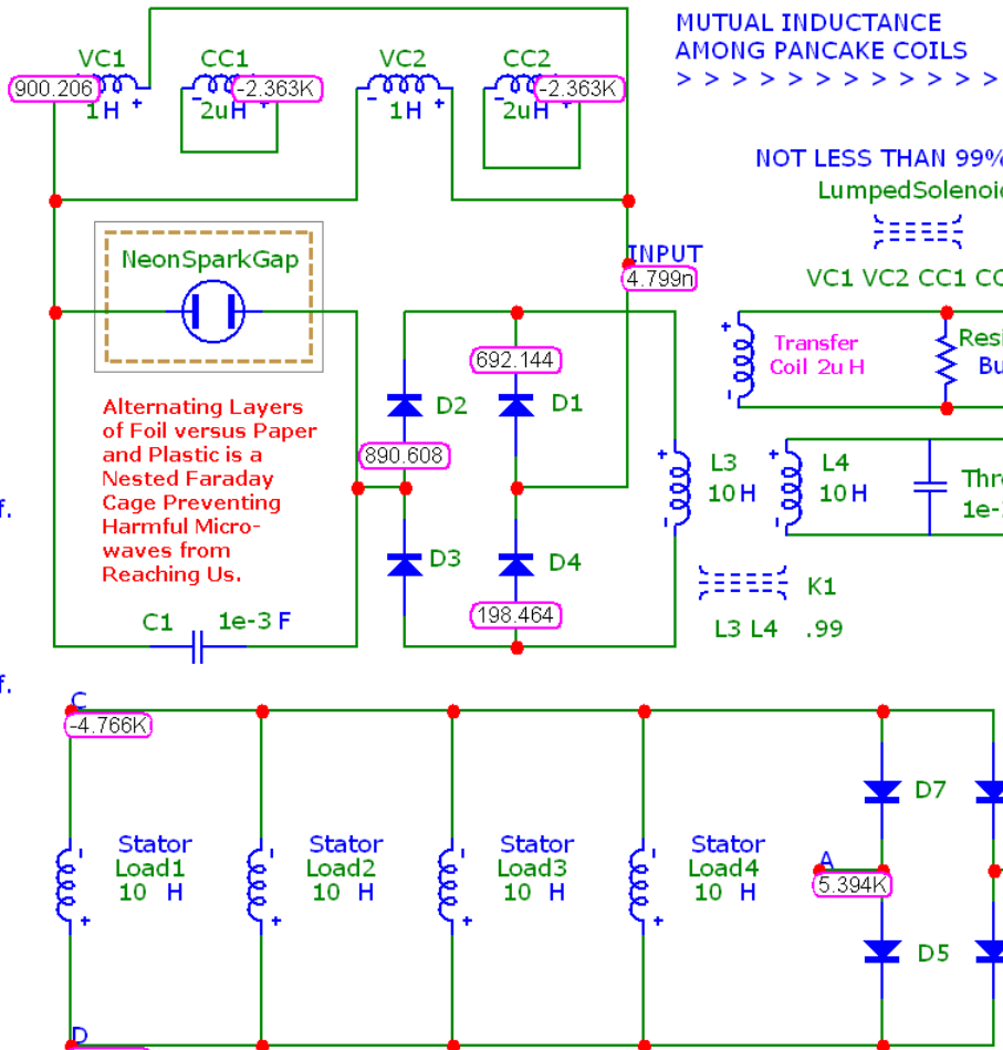
Fig. 38: Nodal Voltages after Two Seconds of Run-Time from Tesla's TriMetal Generator fed by a 3V @ 20k Hz Sine Wave Generator.
