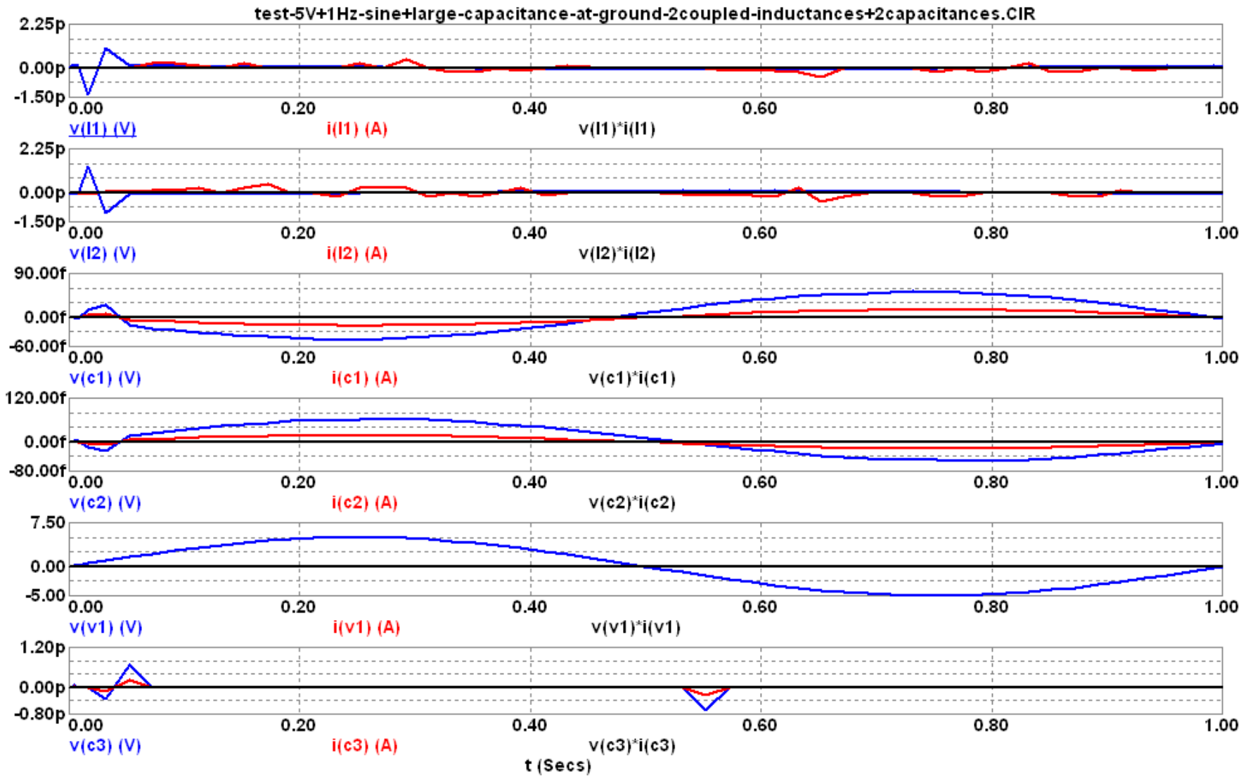
Fig. 25: One Second Output of Two Capacitors, Two Coupled Inductors and One additional Capacitor between Ground and a 5V @ 1Hz Sine Wave Generator.
