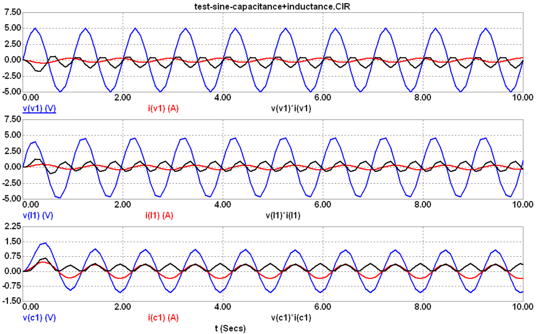
Fig. 10: Output of One Capacitor and One Inductor fed by a Sine Wave Voltage Source.
